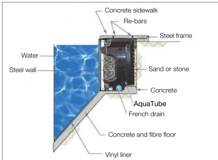
Structural cross-section
